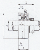
NAFL3 Eccentric locking collar type
